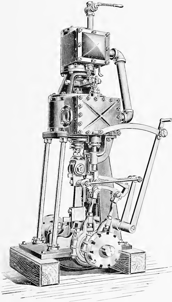
THE MORRIS STEEPLE COMPOUND ENGINE, 8 and 16 by 8.
